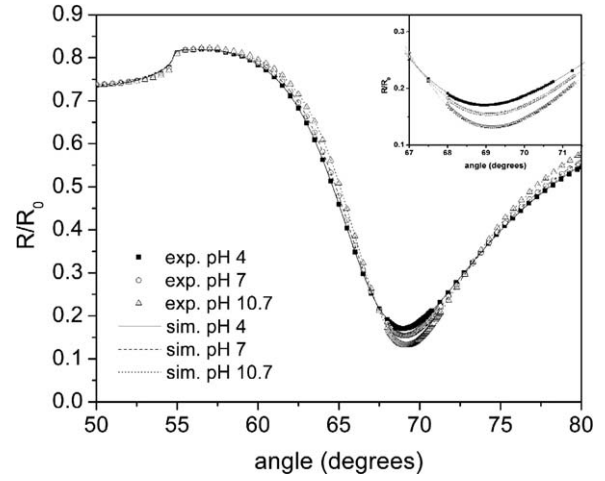
Figure 4. Experimental Angle-Resolved SPR Signals for Three Different pH Conditions
